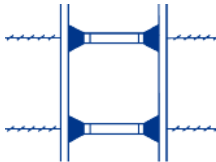
Formwork Ties
